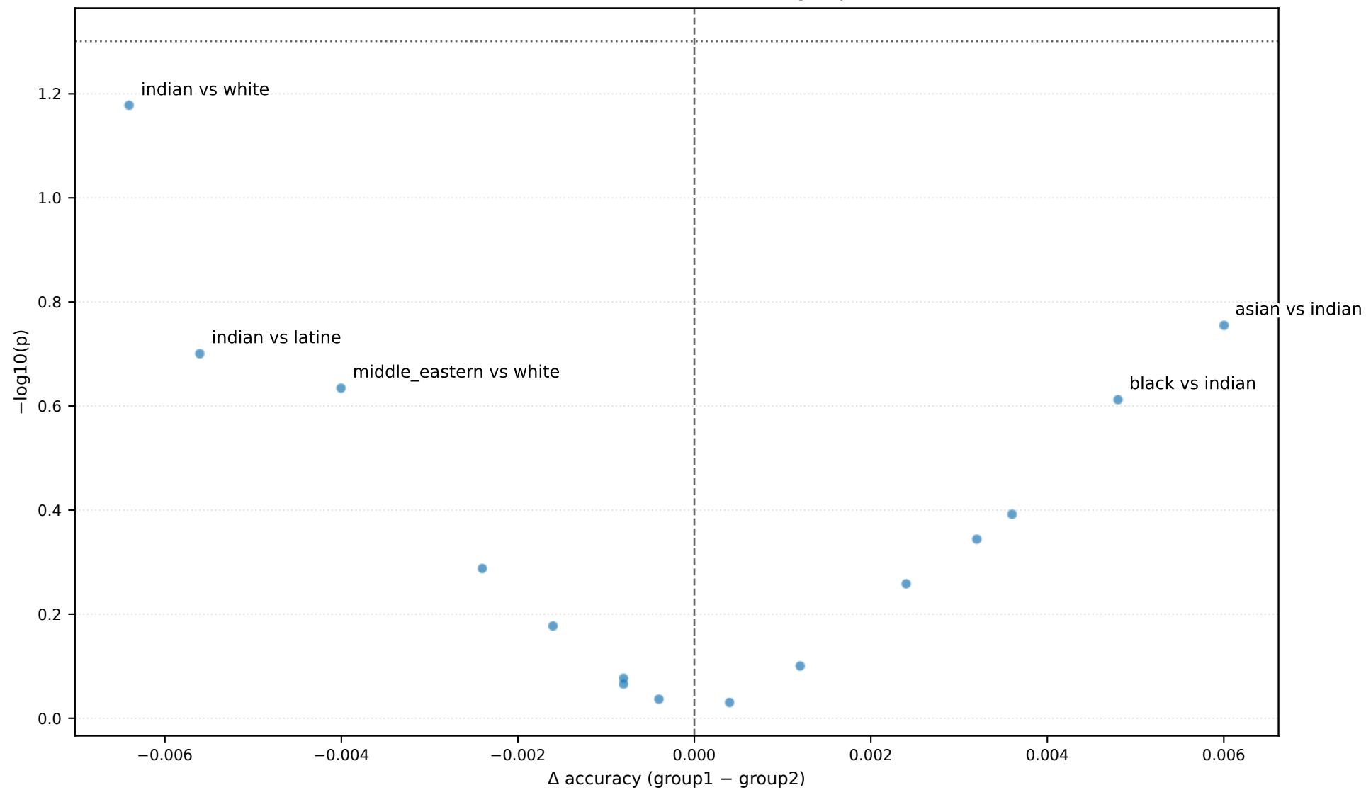
(a) Volcano — Difference vs -\log_{10}(p)
